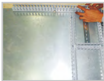
FITTING ASSEMBLY
